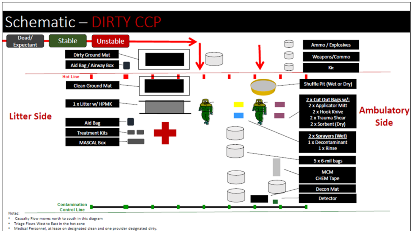
Figure 1. Casualty decontamination schematic.
